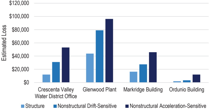
Building Loss from Northridge M6.9 Event
