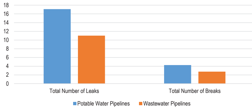
Pipeline Repairs Required After Northridge M6.9 Event
