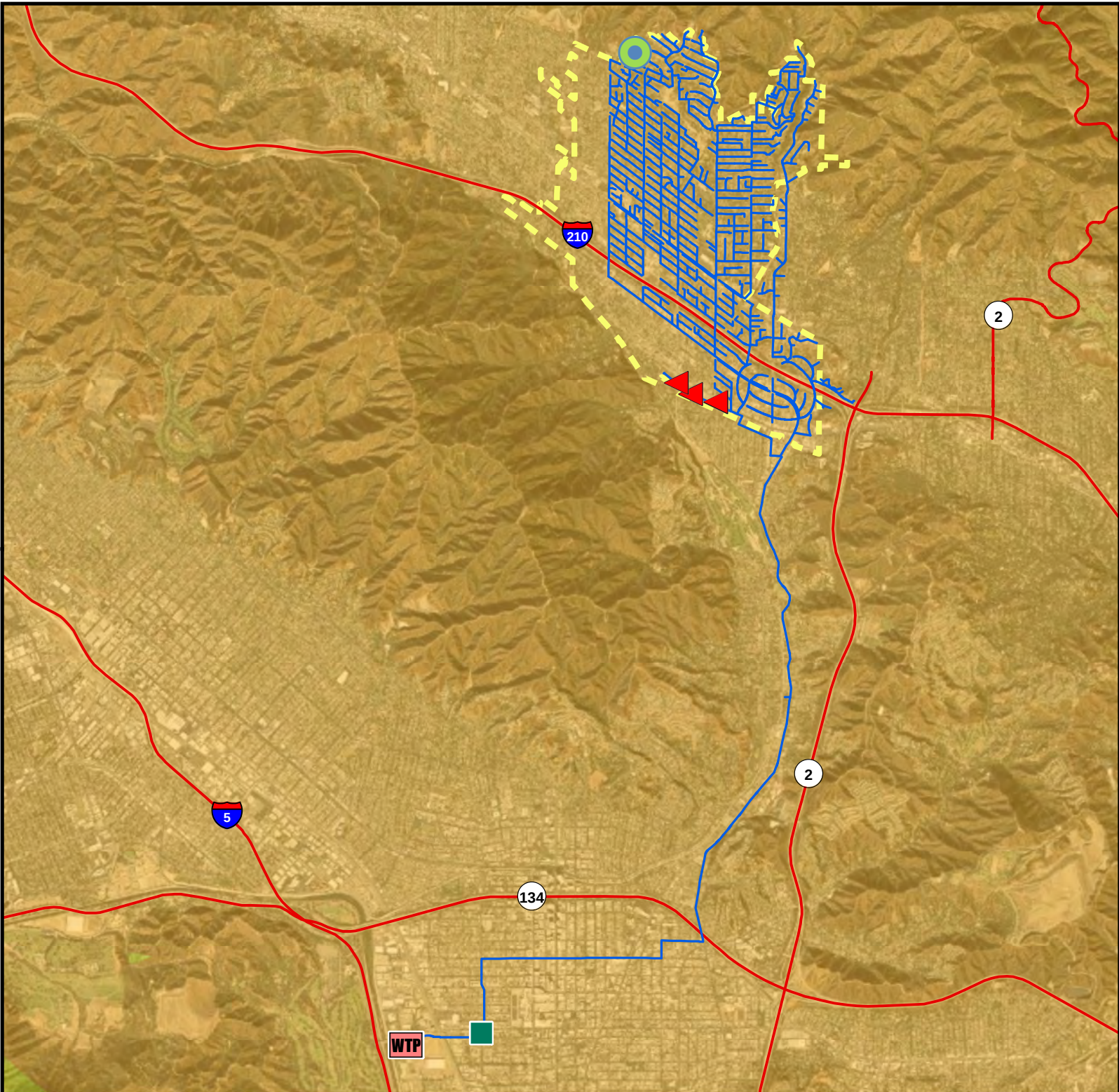
Figure 8-13. Wastewater System - Verdugo M6.9 Earthquake Scenario
