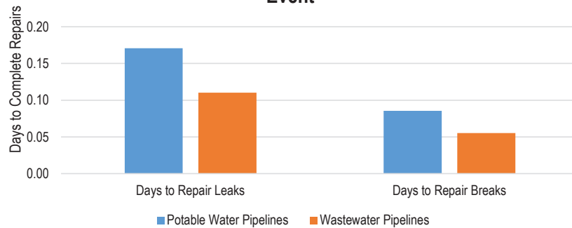
Time to Complete Pipeline Repairs After Northridge M6.9 Event
