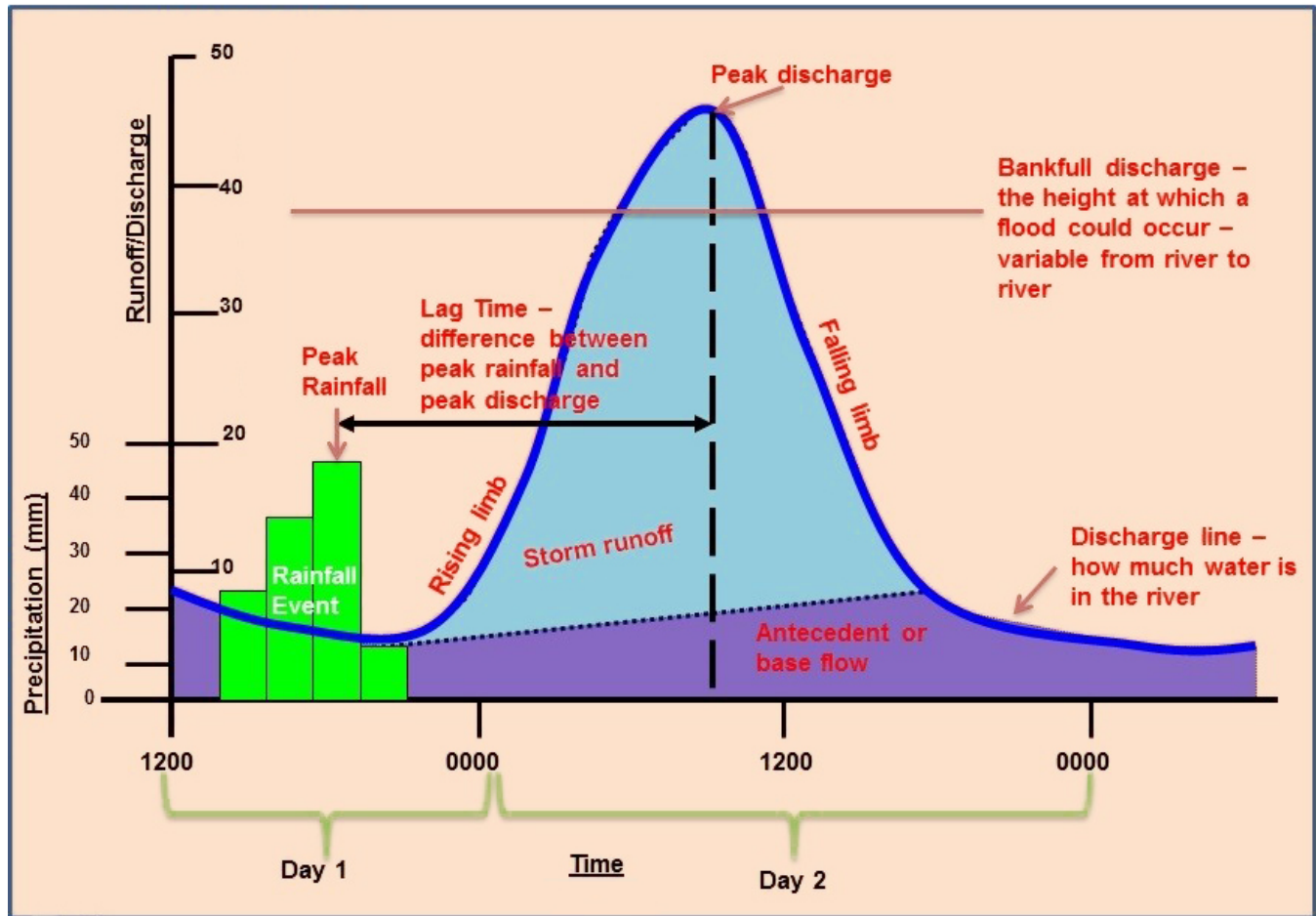
Figure 9-2. Example Hydrograph
